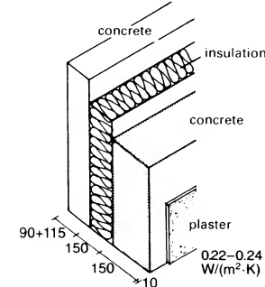
⑤ Double skin concrete 0.22-0.24 W/(m 2 ·K)
